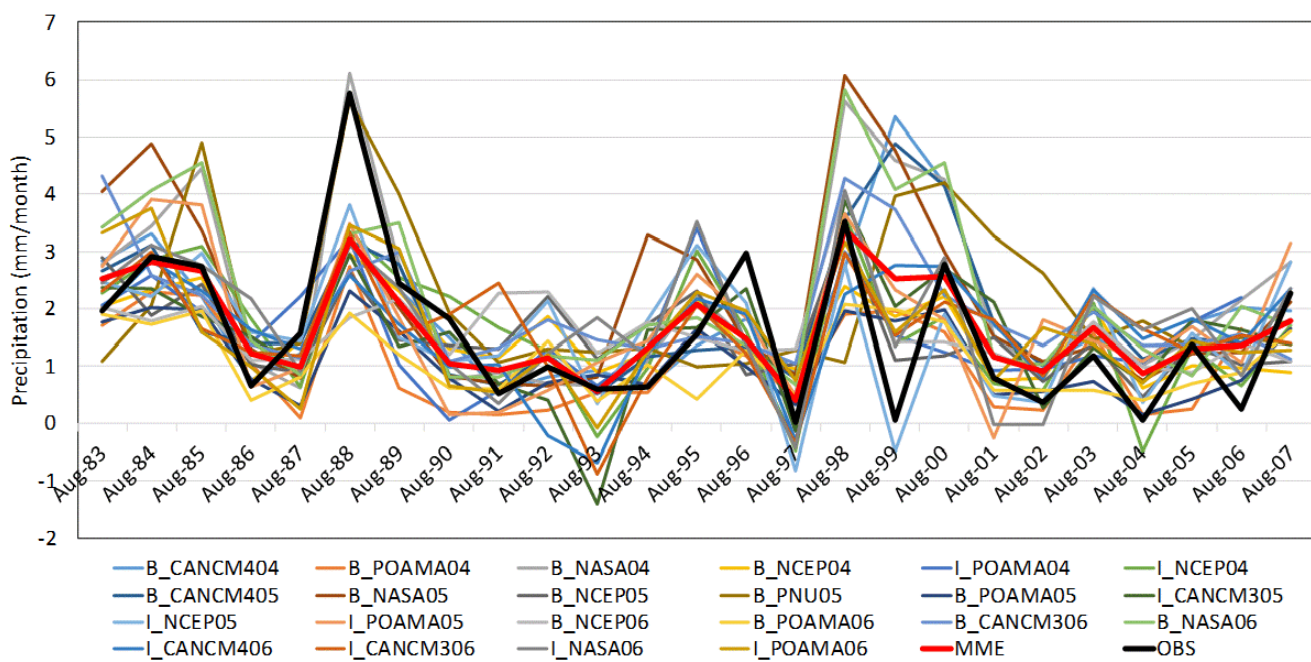
FIGURE 4. Timeseries (left) and scatter plot (right, next page) of monthly precipitation for August issued in April, where B_, M_, C_, I_ indicate SBC, MWR, CIR, ITR downscaling methods, respectively.
